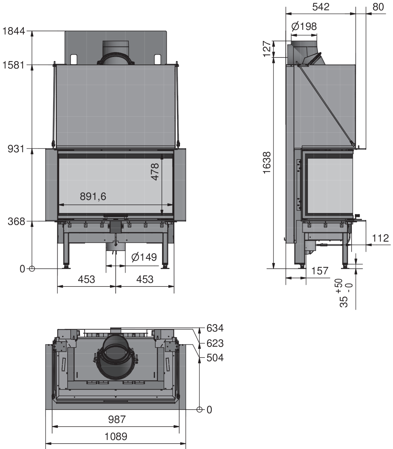
Visio 3 L - With frame
