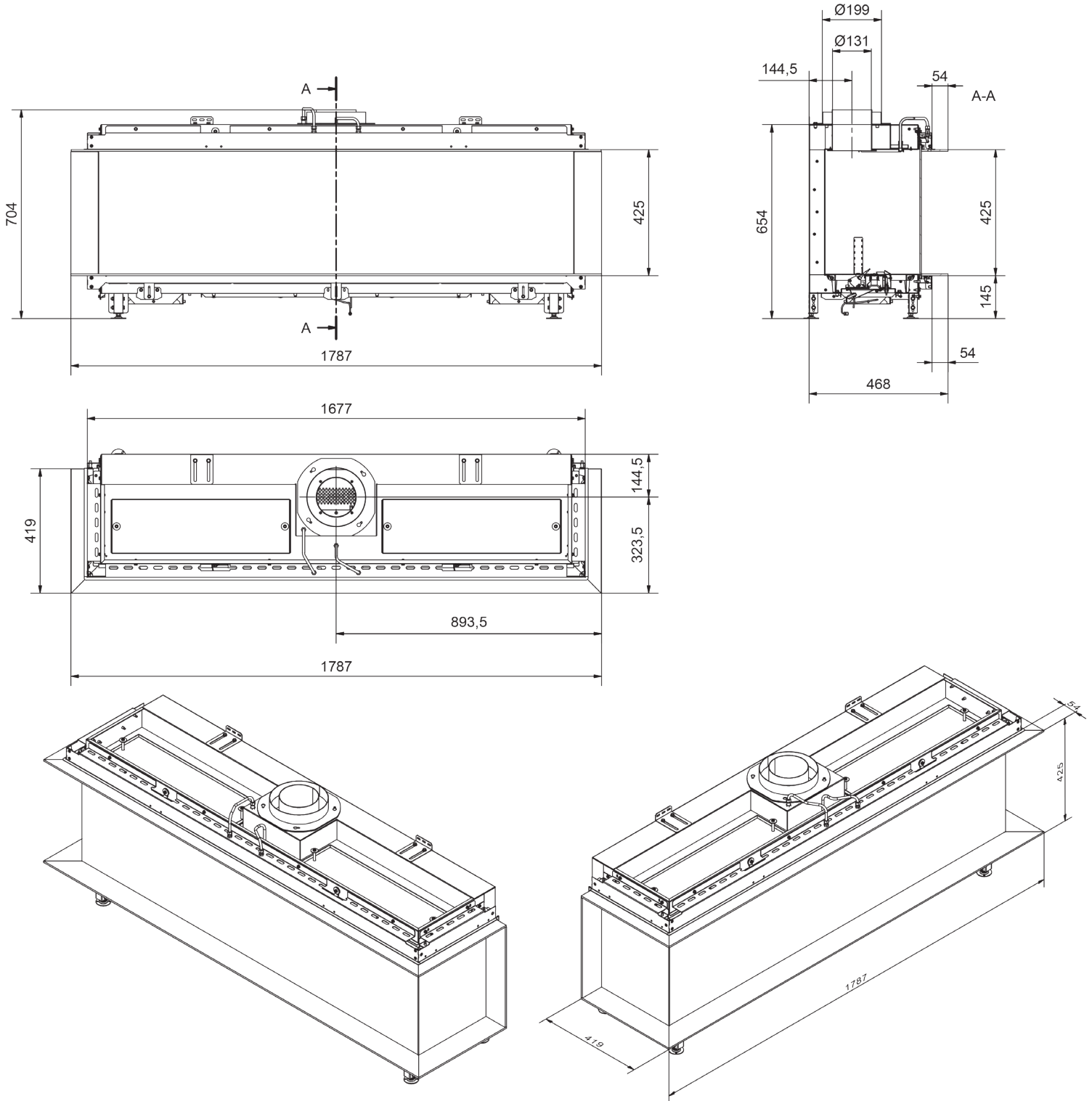
RAIS Visio Gas 160-45-32 3S-6541
